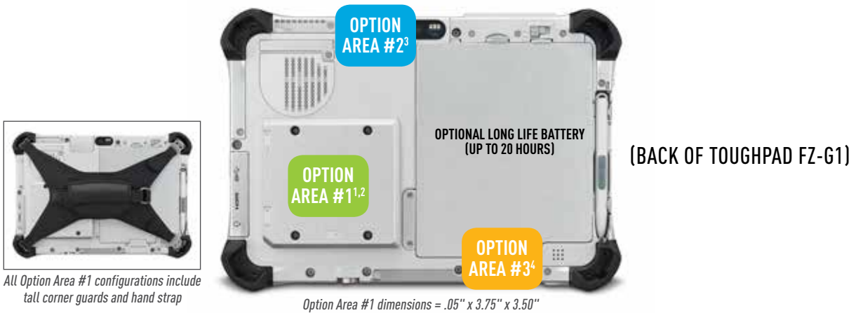
Option Area #1 dimensions = .05" x 3.75" x 3.50"
