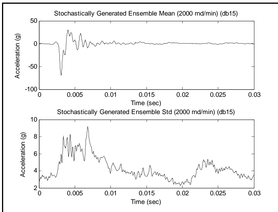
Figure 519.6B-8c. Ensemble and stochastically generated pulse ensemble random component standard deviation (2000 r/min).
