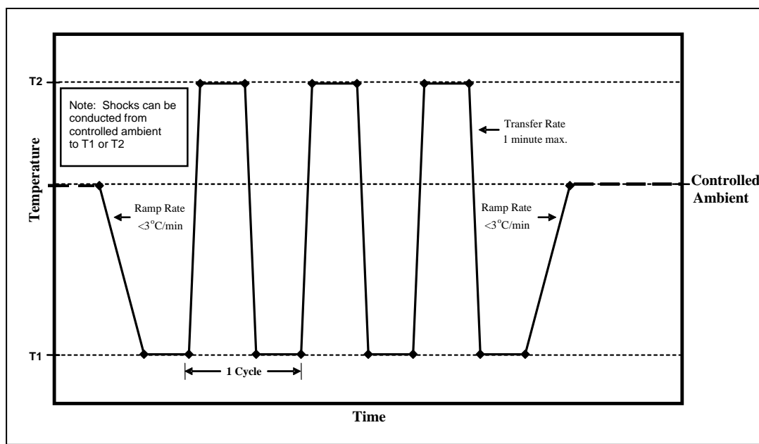
Figure 503.5-3. Multi-cycle shocks.
