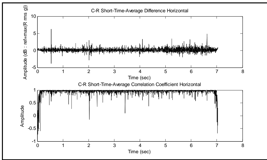
Figure 519.6A-6. STARMS difference between control and reference with cross-correlation estimate. (Difference: \text{ref} = 45.1 \text{ g-rms} / \text{Cross-Correlation} )
